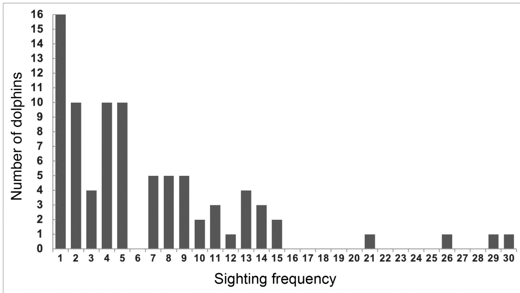
Figure 3. Frequency of sightings ( n = 555 ) for 84 bottlenose dolphins photo-identified in the SF Bay Area from 2007 to 2018
